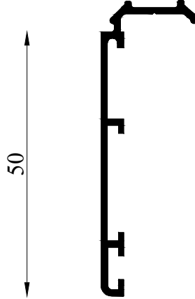
DW 12302 0.302 KG/M IX= 3.88 CM4 IY= 0.22 CM4
