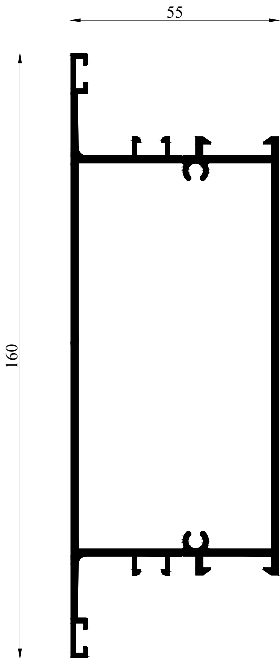
EX 55300 2.295 KG/M IX=178.37 CM 4 IY= 43.57 CM 4
