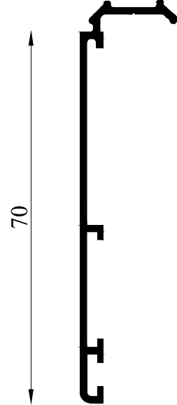
DW 12302/A 0.367 KG/M IX= 8.72 CM4 IY= 0.23 CM4
