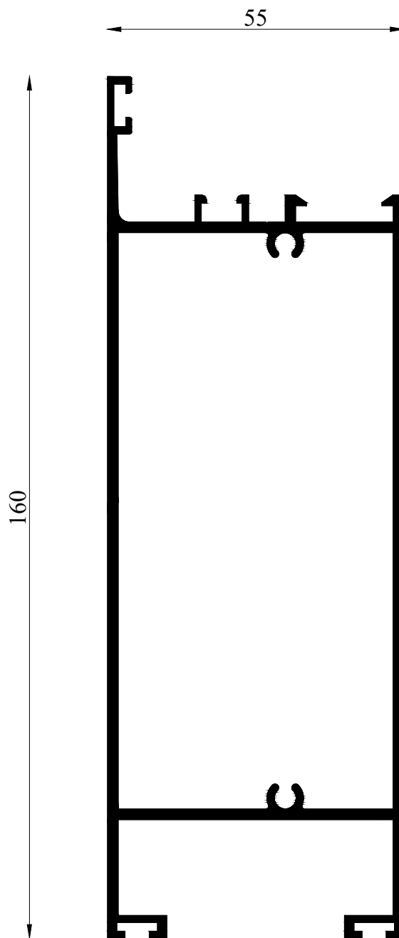
EX 55301 2.433 KG/M IX=216.11 CM 4 IY= 48.34 CM 4
