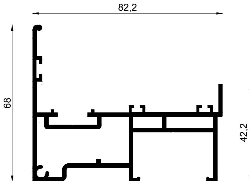
VS 10314 1.161 KG/M IX: 23.79 CM 4 IY: 3.96 CM 4
