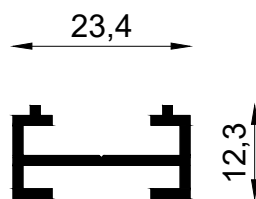
VS 10323 0.213 KG/M IX: 0.0898 CM4 IY: 0.6192 CM4
