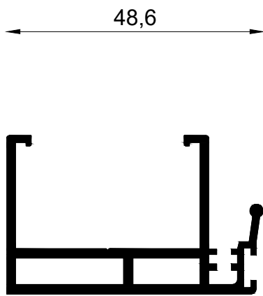
VS 10312 0.783 KG/M IX: 2.0699 CM4 IY: 7.3271 CM4
