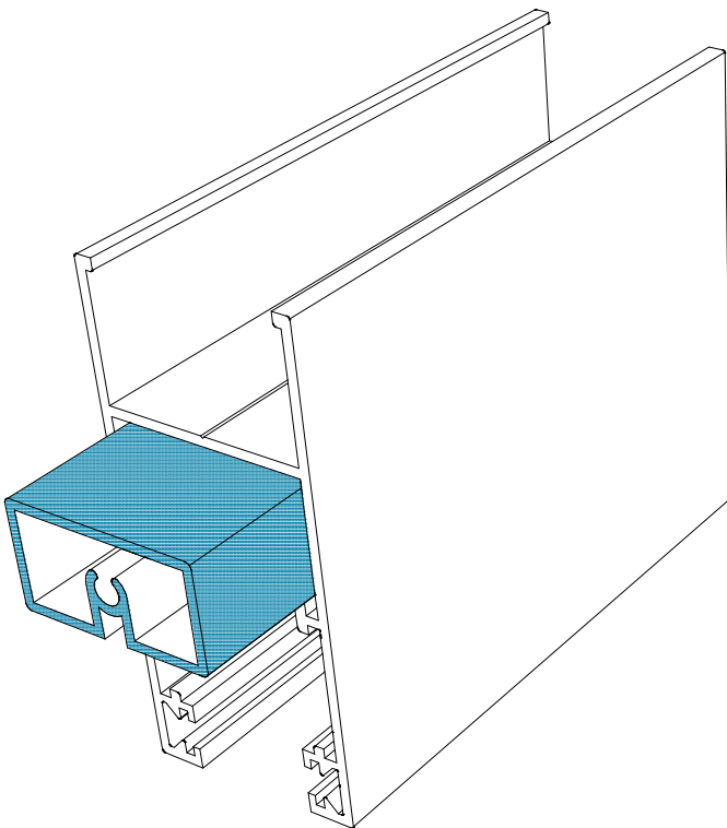
Insert profile VS 10322 in sash profile VS 10200
