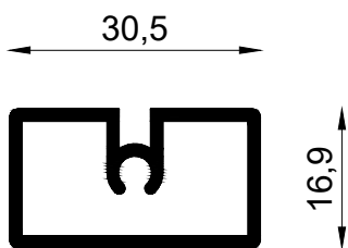
VS 10322 0.429 KG/M IX: 0.61 CM4 IY: 1.58 CM4
