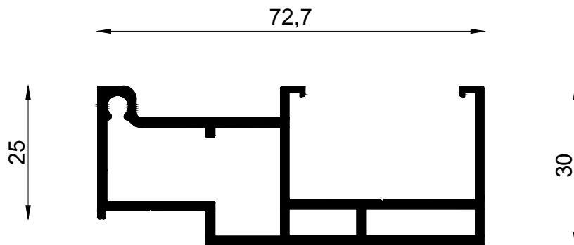
VS 10314 1.161 KG/M IX: 23.79 CM 4 IY: 3.96 CM 4
